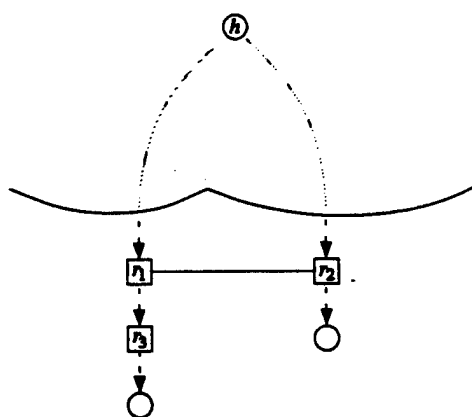
(c) extended reverse-path forwarding
