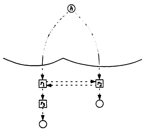
(b) basic reverse-path forwarding
